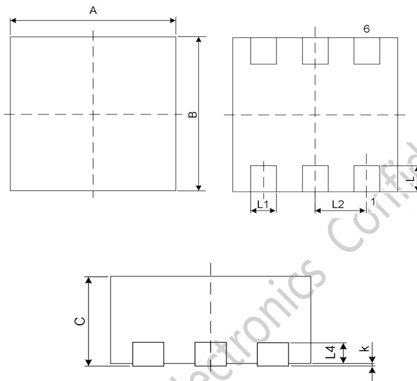
DFN1.6×1.6-6
