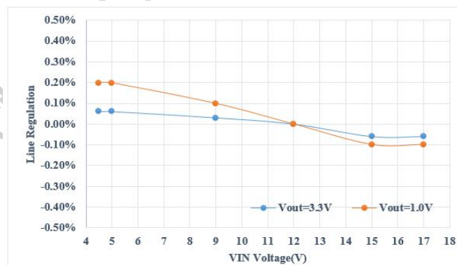
Figure4 Line Regulation I_{out}=1\text{A}
