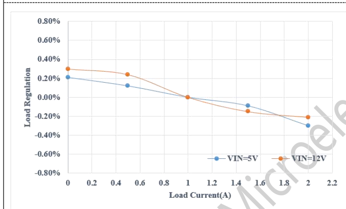
Figure3 Load Regulation
