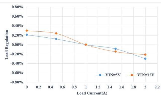
Figure3 Load Regulation
