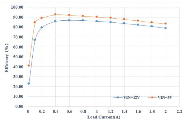
Figure2 1.8V Output Efficiency
